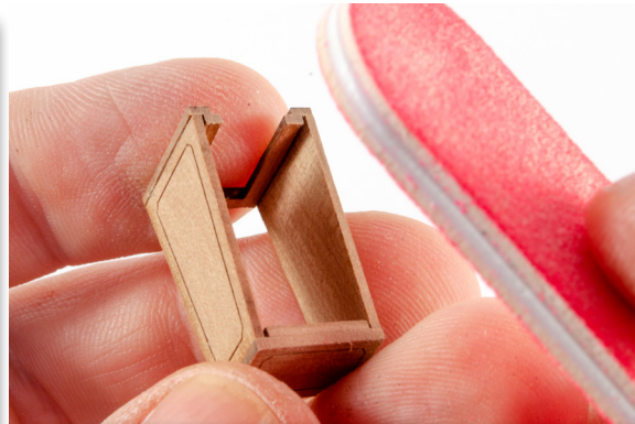
142. When the assembly is thoroughly set, sand the upper and lower sides so all edges are flush with each other.
