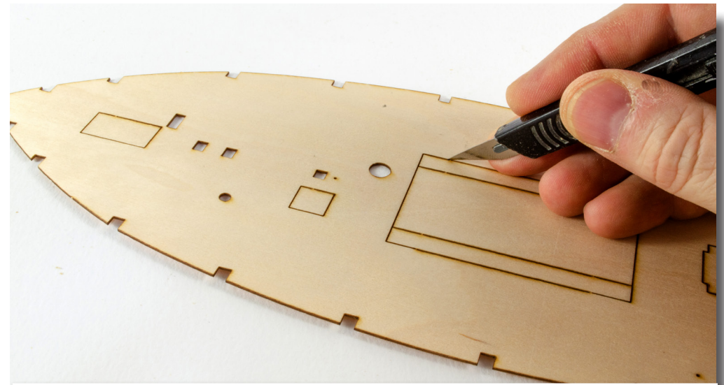
20. You have two deck parts in your kit. Take the plain one without the laser-engraved planking and using a sharp knife, remove the square and rectangular sections from it by cutting through the tabs. Please retain the larger rectangular section for later in the build.
