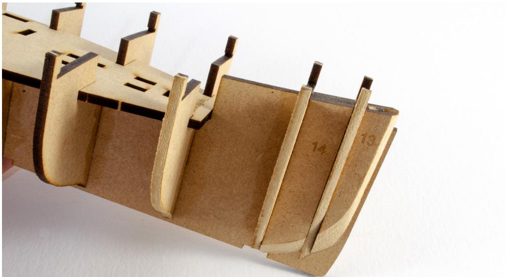
18. You must now do the same for the bow by gluing parts 13 and 14 into place. As before, make sure that the top of these sit flush with the top of the false keel. Repeat on both sides of the bow.
