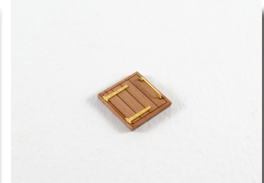
118, 119&120 Remove the Deck Hatch Combing (part 69) and the Deck Hatch Lid (part 70) from the 1mm pear sheet. Also remove two Door Hinge (PE-7) and a Hatch Handle (PE-6) from the photo-etch sheet and assemble as shown. Install the finished unit to the deck in the correct orientation.
