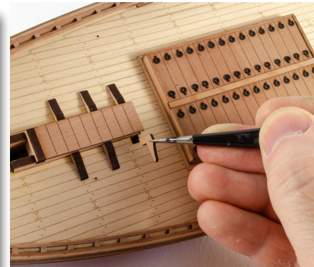
116. Remove the six Fore Mast Opening Side Checks (parts 34) from the 3mm pear sheet and glue into the positions shown.
