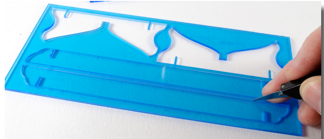
84, 85&86 Time for a change of materials now as we make the acrylic stand. Using a very sharp knife, cut through the tabs holding the parts in place and trim away any excess on the parts. Both sides of the parts are covered in a protective film and you need to peel this away. Now clip the stand together. If the parts are a little tight, don't force them, but very gently file the inside of the slots and test fit so they go together snugly. Note that the parts have a front and rear, so familiarise yourself with how the hull sits on the stand.
