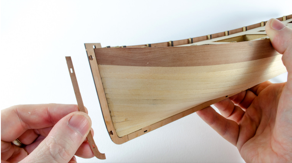
61&62 Now glue the prow rabbet pattern (part 52) to the prow, and clamp until the glue has set.
