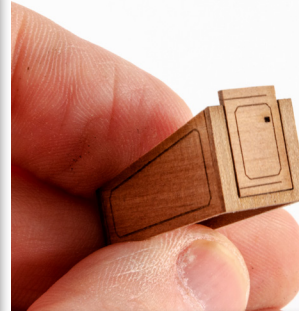
143. Glue the Aft Companionway Door (part 64) into position. Note the orientation.
