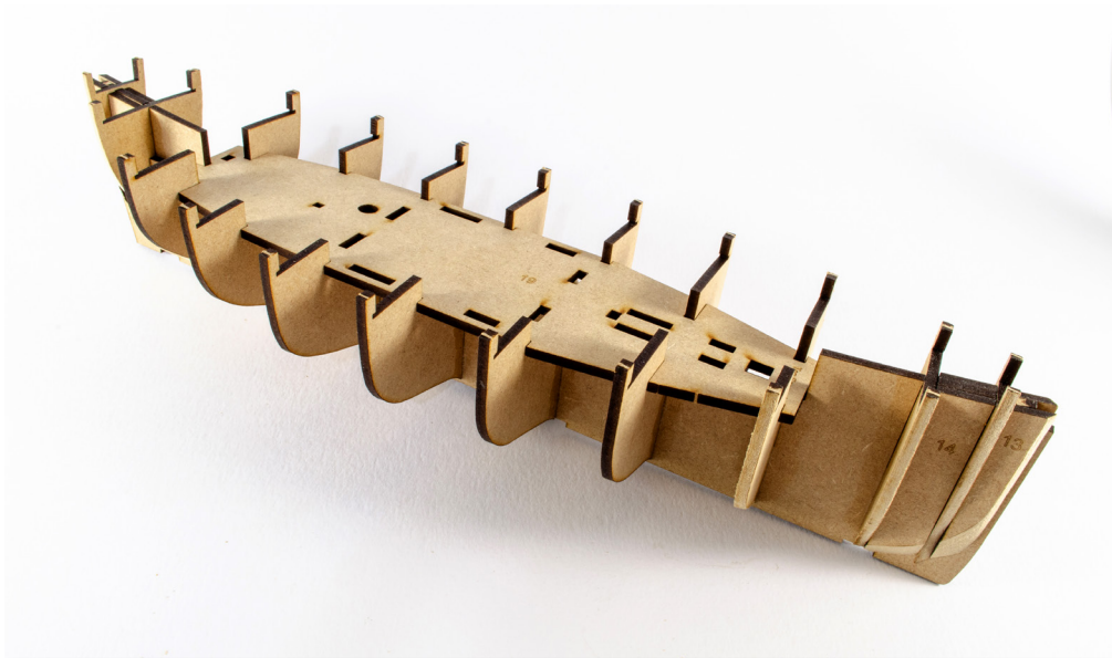
19. Your hull skeleton should now look like this. Again, leave the glue to set before continuing.
