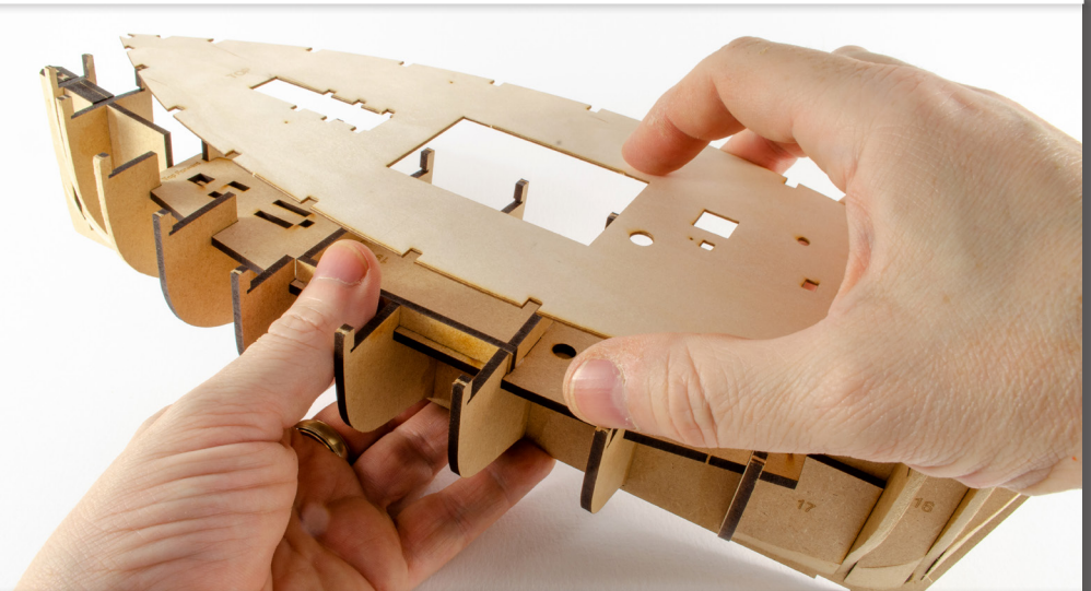
25. The deck has been designed so that it clicks perfectly into place, being held at the edge of the bulkheads by a small recess that means you don't need to pin it whilst it dries. Our experience has shown that once you fit the deck, it takes some effort to remove. At this point, you can, if you wish, run glue over the bulkheads in readiness to fit the deck. However, we choose to fit it without glue at this stage.
