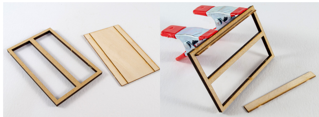
104&105 Take the Fish Hatch Frame (part 22) from the MDF sheet, and the Fish Hatch Inner Combing part that you removed from the middle of the laser engraved deck. Remove the two outer thin strips and glue them to the inside outer edge of the fish hatch frame.
