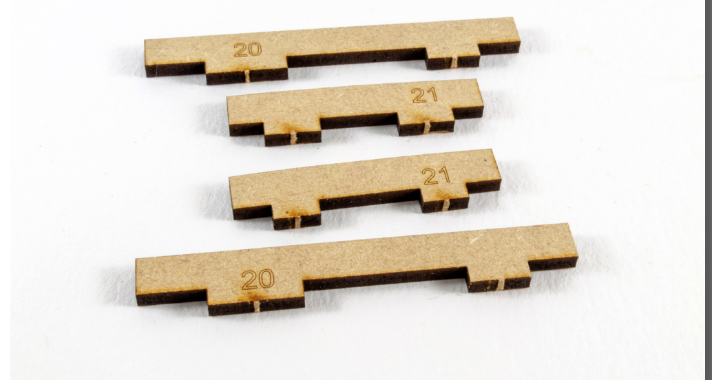
21. Cut parts 20 (x2) and 21 (x2) from the 3mm MDF sheet. Note that parts 21 actually have different length tabs and are curved on top. The curve forms part of the deck's curve (camber) when installed.
