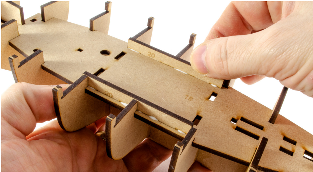
22. Glue the two part 20 pieces into position. Each has tabs of different lengths and they will fit into the model only a certain way. This photo shows you how these will look when fitted.
