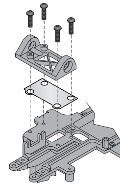
Using Belt Adjustment Shims
