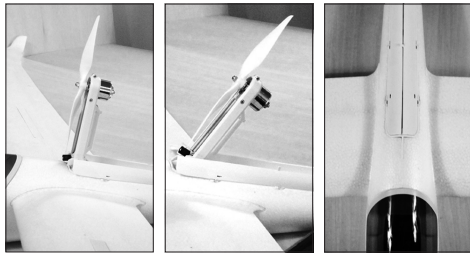
Fig. 11 – 1.1 Retractable power unit mixer module:
