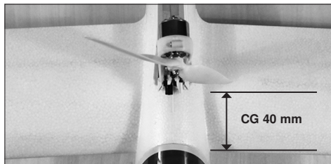
Centre of Gravity 40 mm with the power unit extended.
