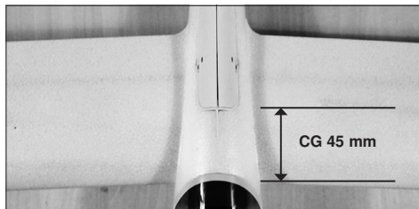
Centre of Gravity 45 mm with the power unit retracted.
