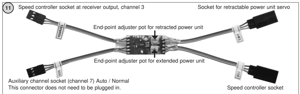
Fig. 11 – 1.1 Retractable power unit mixer module:
