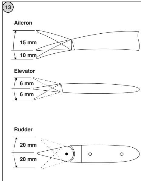
Fig. 13 Control surface travels
