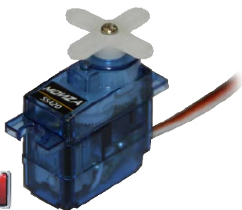
SSA20 Servo MONZA 2,0kg.cm 0,10s/60° 4,8-6V
