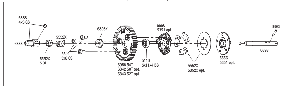
Slipper Clutch Assembly
